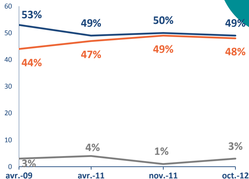
Evolutions
